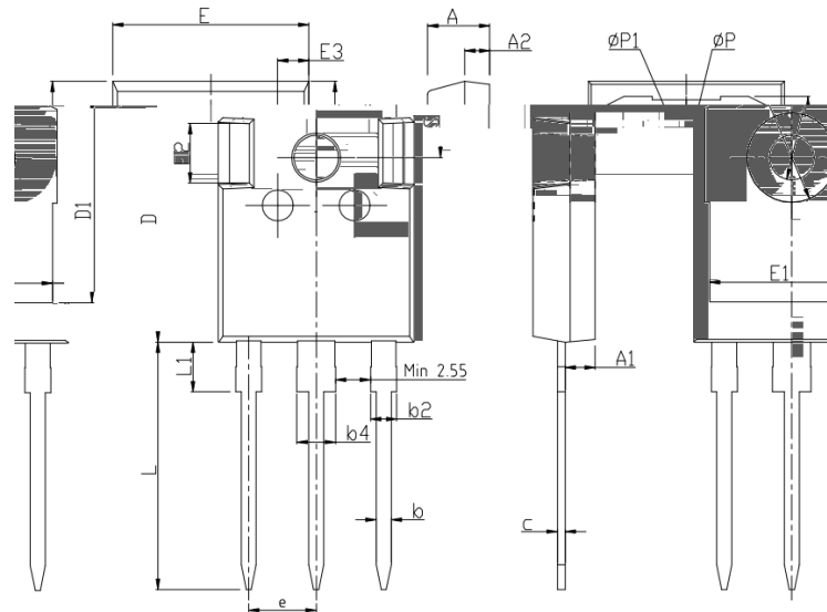
COMMON DIMENSIONS
