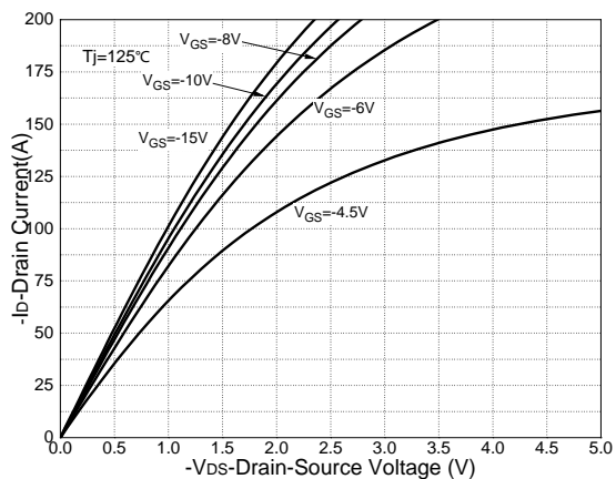
Figure 15: Output Characteristics 125
