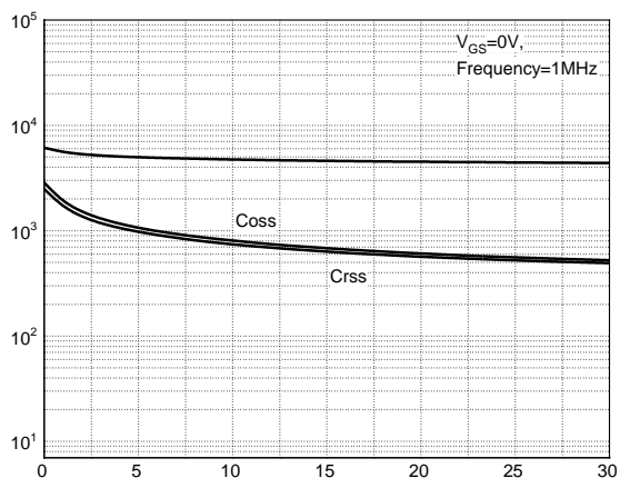
Figure 9: Capacitance Characteristics
