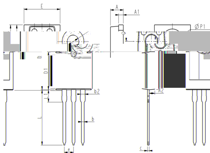
COMMON DIMENSIONS
